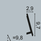
SX179 DIAGONAL 200 x 9,7 x 2,9 cm Duopolymer ® Designed by Orio Tonini
