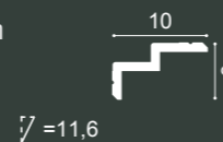
1 C390 STEPS 200 x 6 x 10 cm Purotouch® Designed by Orio Tonini
