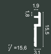
C395 STEPS 200 x 15,5 x 3,1 cm Purotouch® Designed by Orio Tonini
